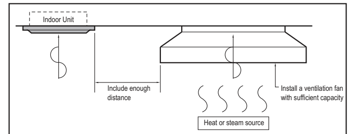
Figure 84: Installing Near a Heat or Steam Source.
