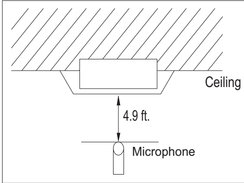
Figure 37: Sound Pressure Measurement Location.
