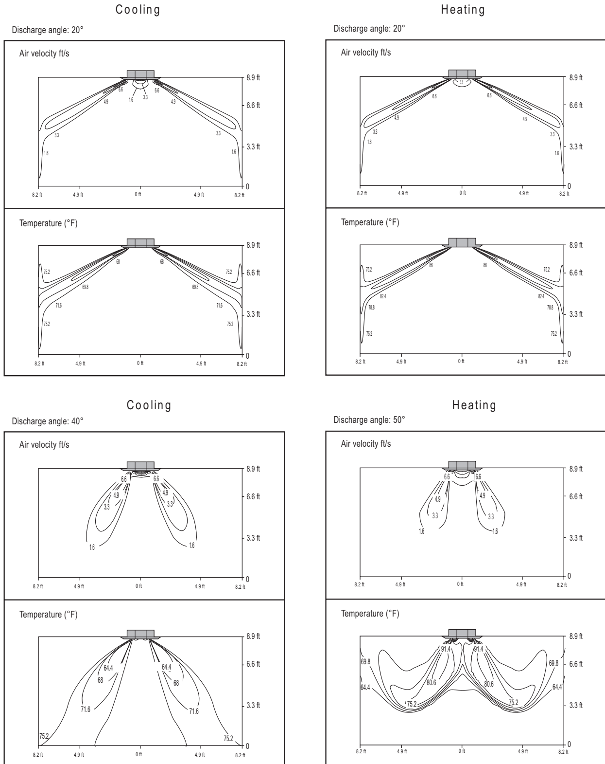
Figure 55: ARNU093TRD4.
