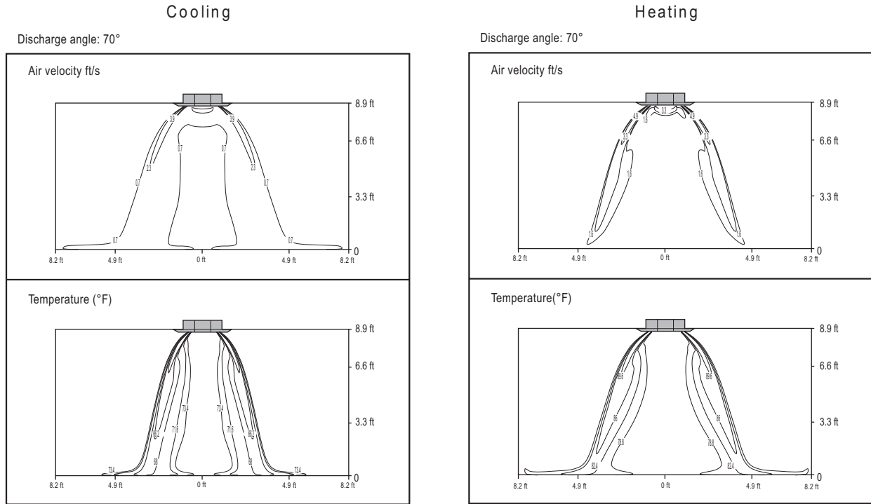
Figure 52: ARNU053TRD4, continued.
