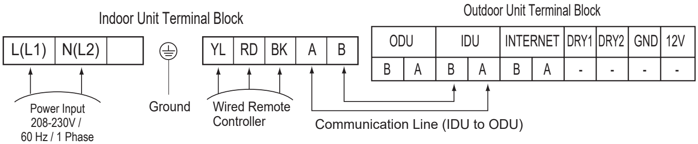
Figure 97: TS Frame Wiring / Cable Connections.
