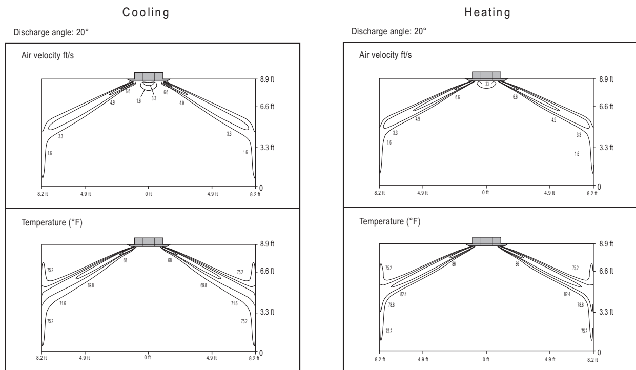
Figure 53: ARNU073TRD4.
