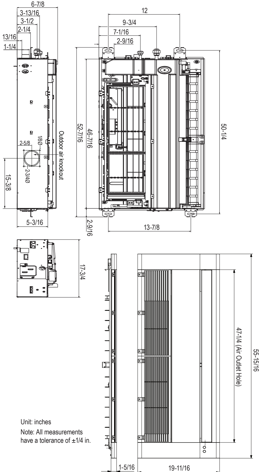
Figure 4: ARNU183TTD4, ARNU243TTD4 Dimensions (PT-UTC Grille).
