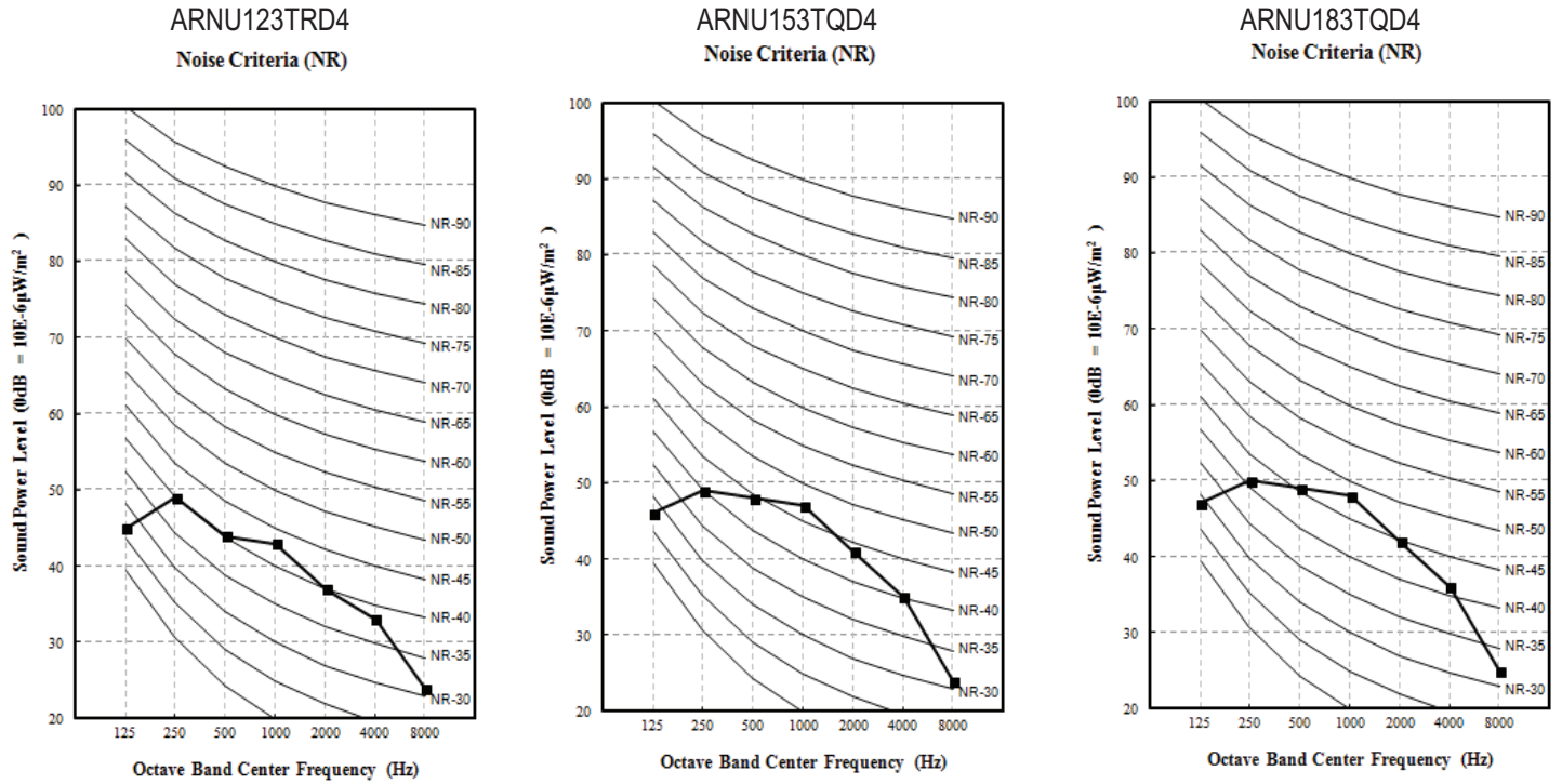
Figure 45: ARNU123TRD4, ARNU153TQD4, and ARNU183TQD4 Sound Power Level Diagrams.
