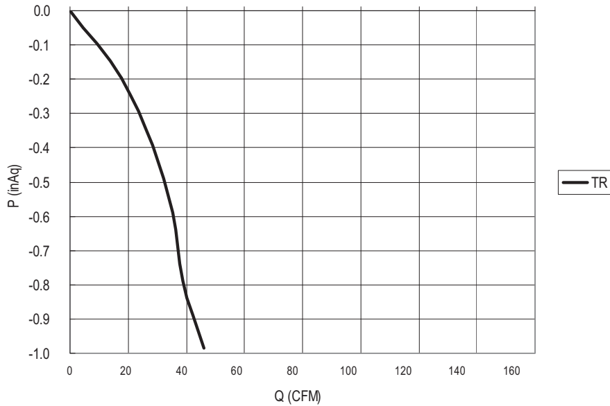
Figure 80: TQ Frame Fresh Air Ventilation.
