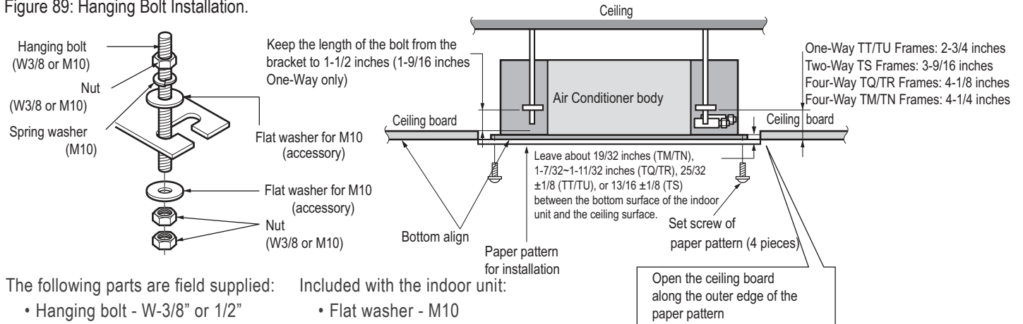
Figure 89: Hanging Bolt Installation.
