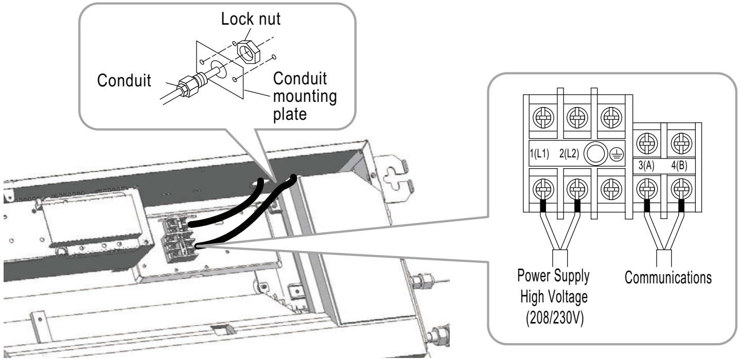
Figure 95: Typical TT, TU Frame Wiring / Cable Routing.
