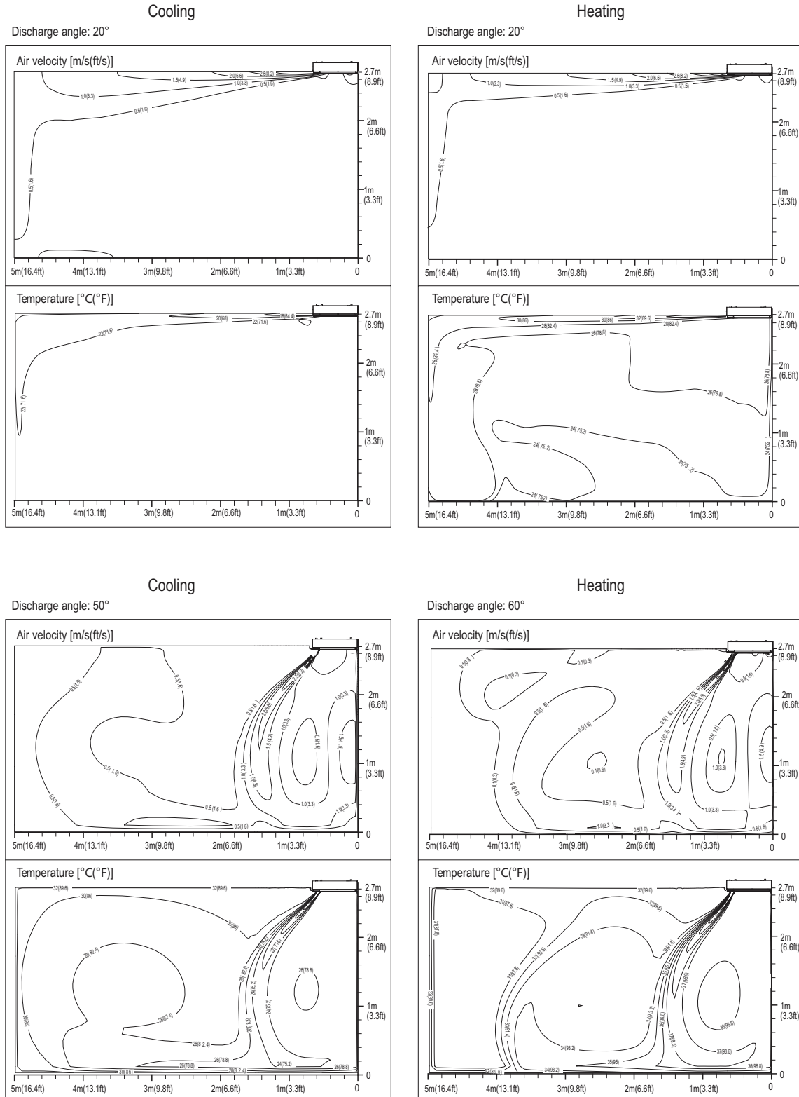
Figure 16: ARNU123TUD4.
