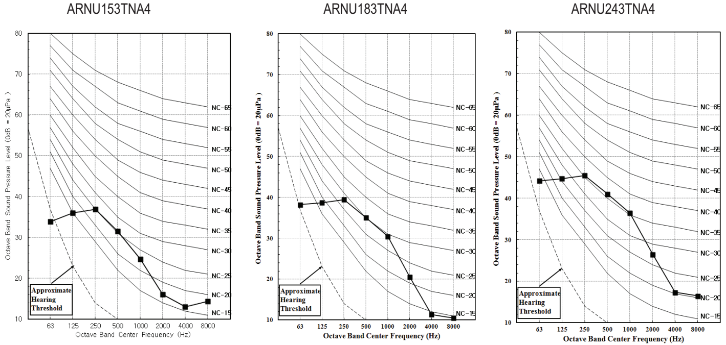
Figure 41: ARNU153TNA4, ARNU183TNA4, and ARNU243TNA4 Sound Pressure Level Diagrams.
