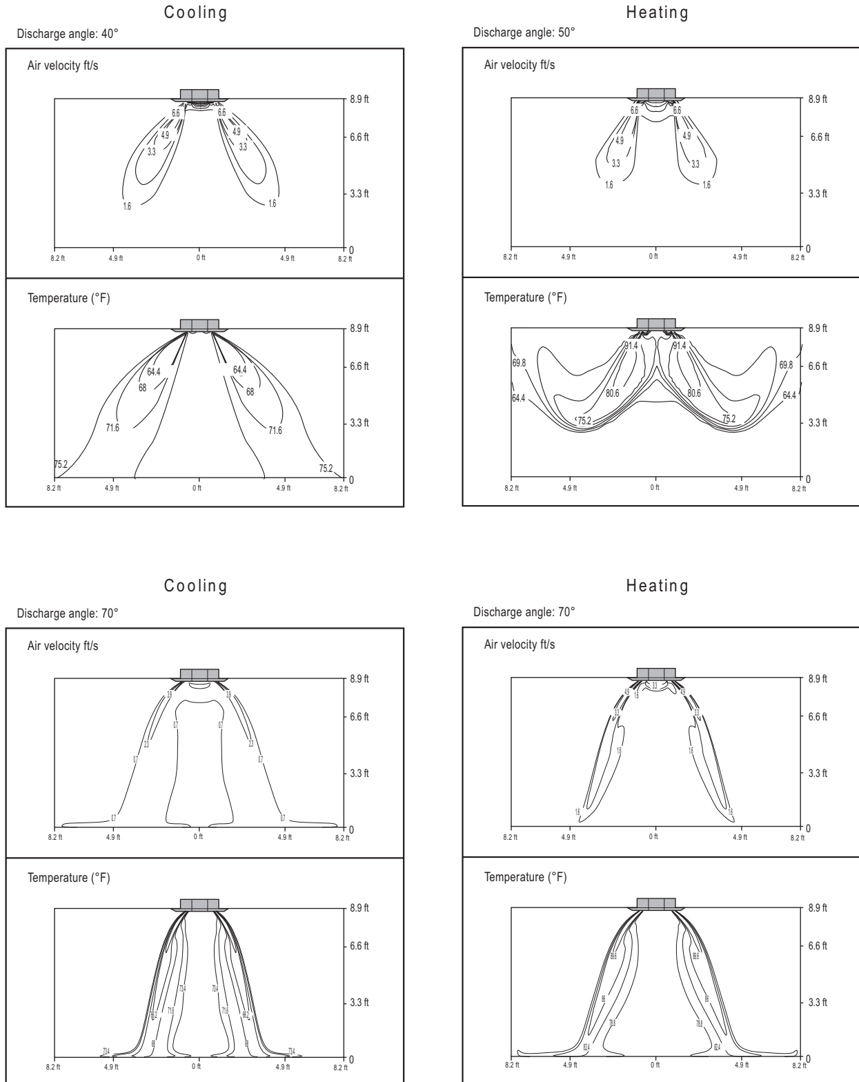
Figure 54: ARNU073TRD4, continued.
