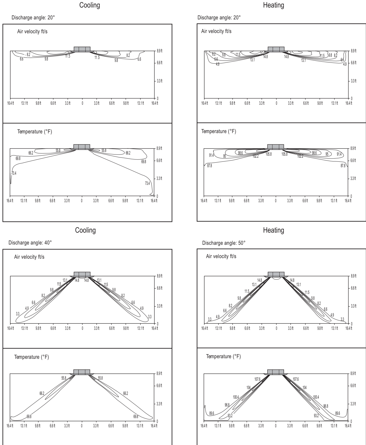
Figure 73: ARNU363TMA4.
