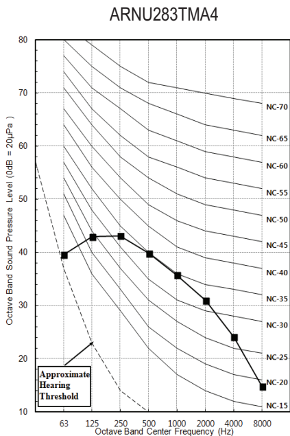
Figure 42: ARNU283TMA4 Sound Pressure Level Diagram.
