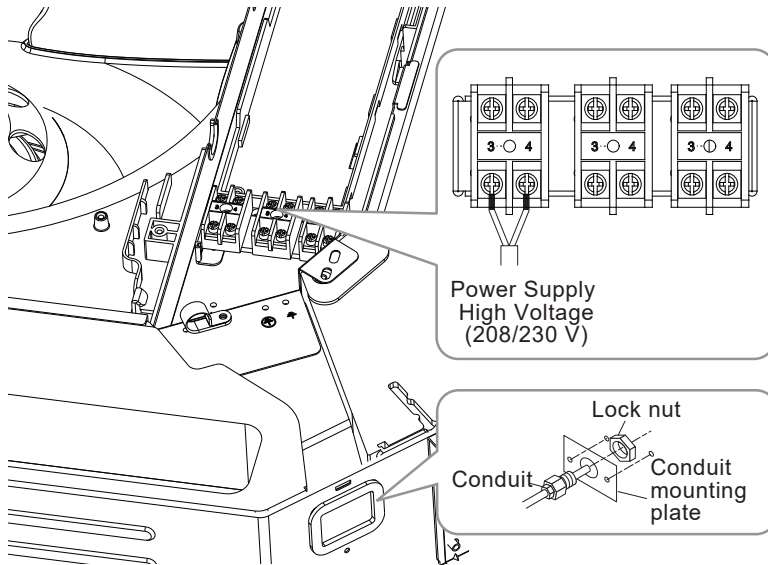
Figure 99: Typical Four-Way Cassette Wiring / Cable Routing, Side View.
