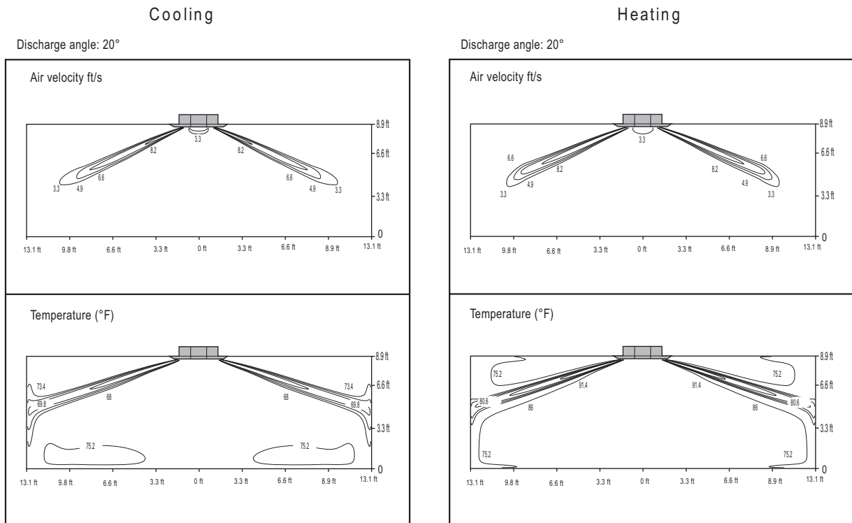
Figure 61: ARNU183TQD4.
