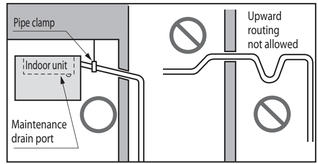
Figure 92: Drain Piping Slope.
