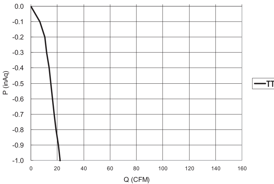
Figure 23: TT Frame Fresh Air Ventilation.
