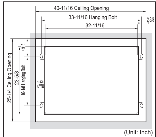
Figure 86: Ceiling Opening / Hanging Bolt Locations for Two-Way Ceiling Cassette Indoor Units.
