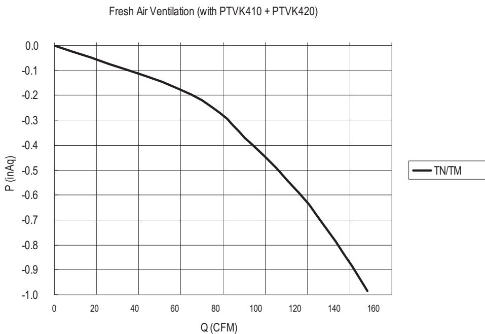
Figure 82: TN and TM Frame Fresh Air Ventilation with PTVK410 + PTVK420 Accessories.
