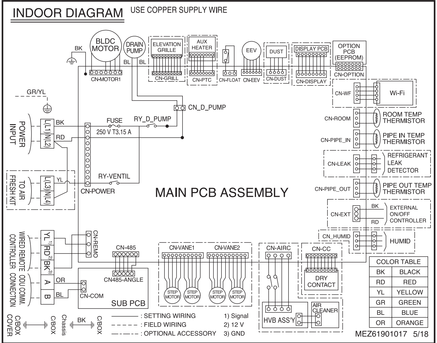
Figure 35: ARNU073TNA4, ARNU093TNA4, ARNU123TNA4, ARNU153TNA4, ARNU183TNA4, ARNU243TNA4, ARNU283TMA4, ARNU363TMA4, ARNU423TMC4, ARNU483TMC4 Wiring Diagram.
