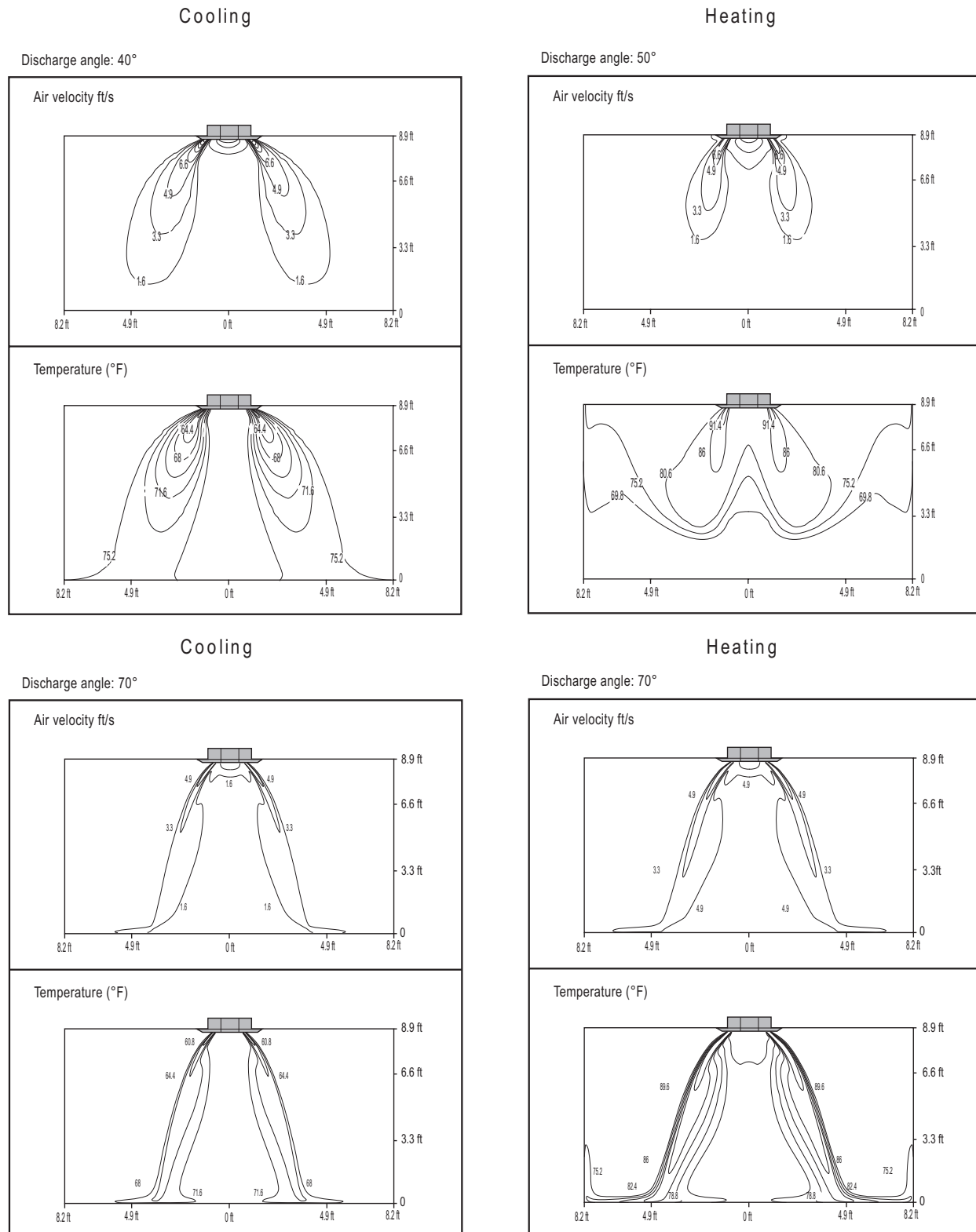
Figure 58: ARNU123TRD4, continued.
