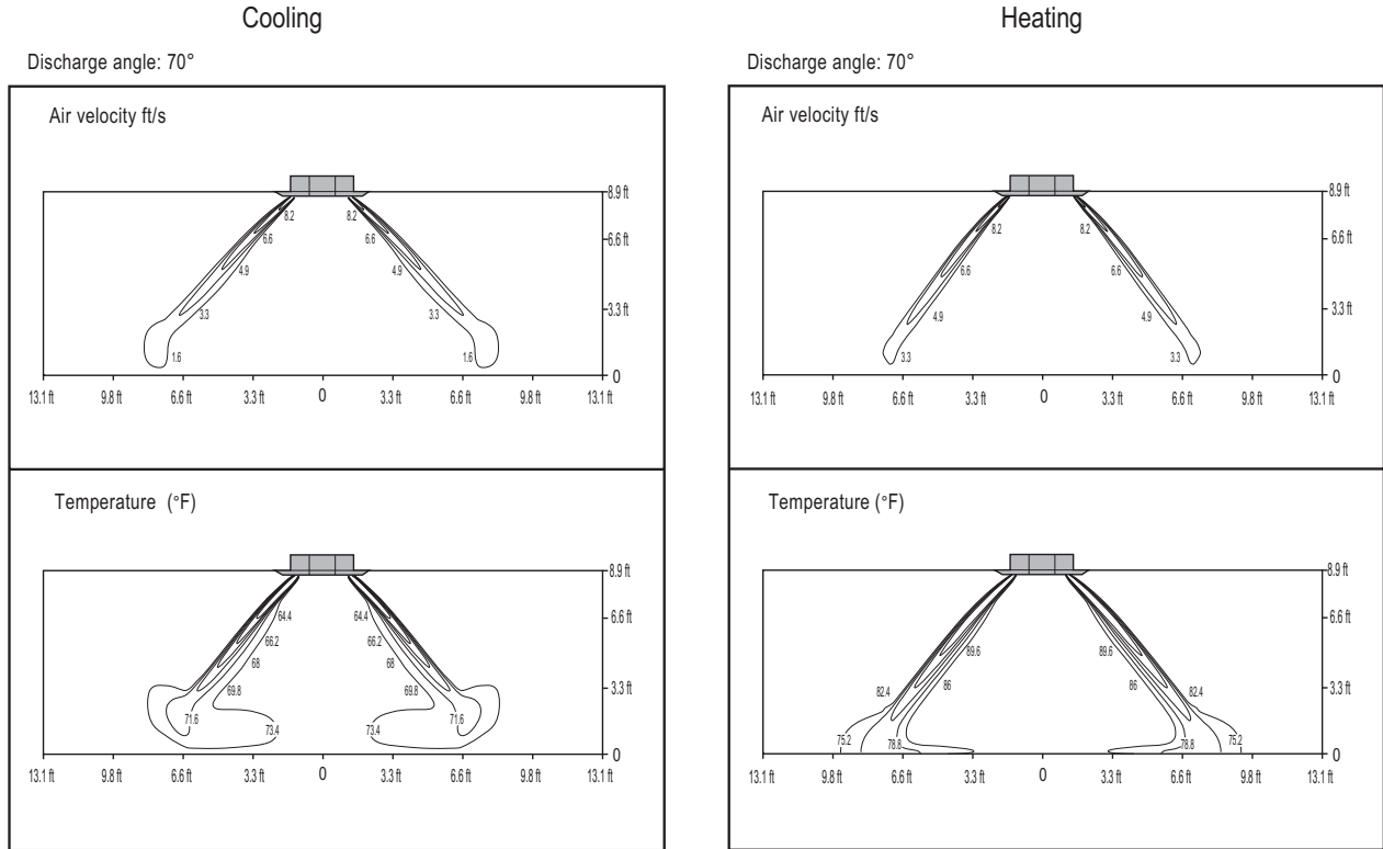
Figure 69: ARNU243TNA4.
