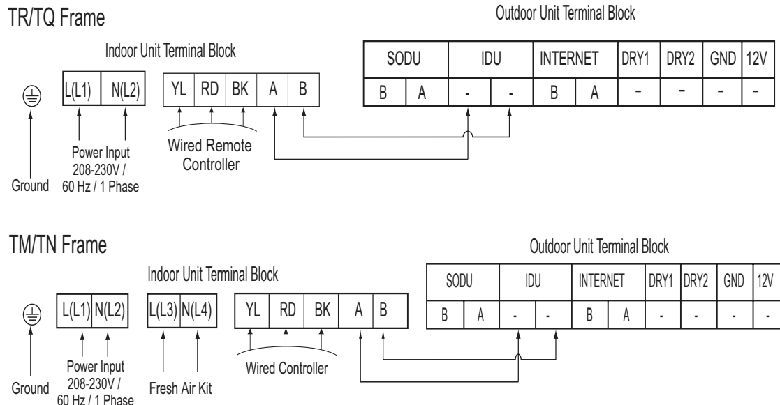
Figure 100: Four-Way Ceiling-Cassette Wiring / Cable Connections.
