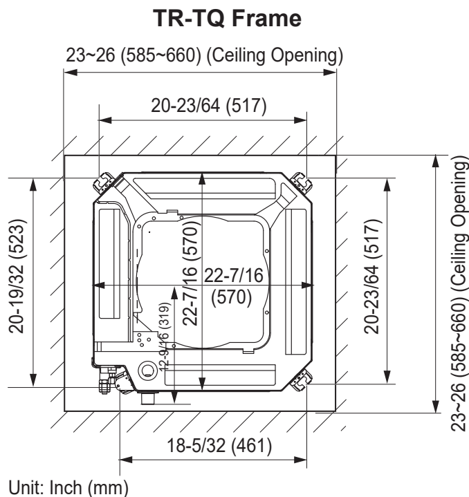
Figure 87: Ceiling Opening / Hanging Bolt Locations for Four-Way Ceiling Cassette Indoor Units.
