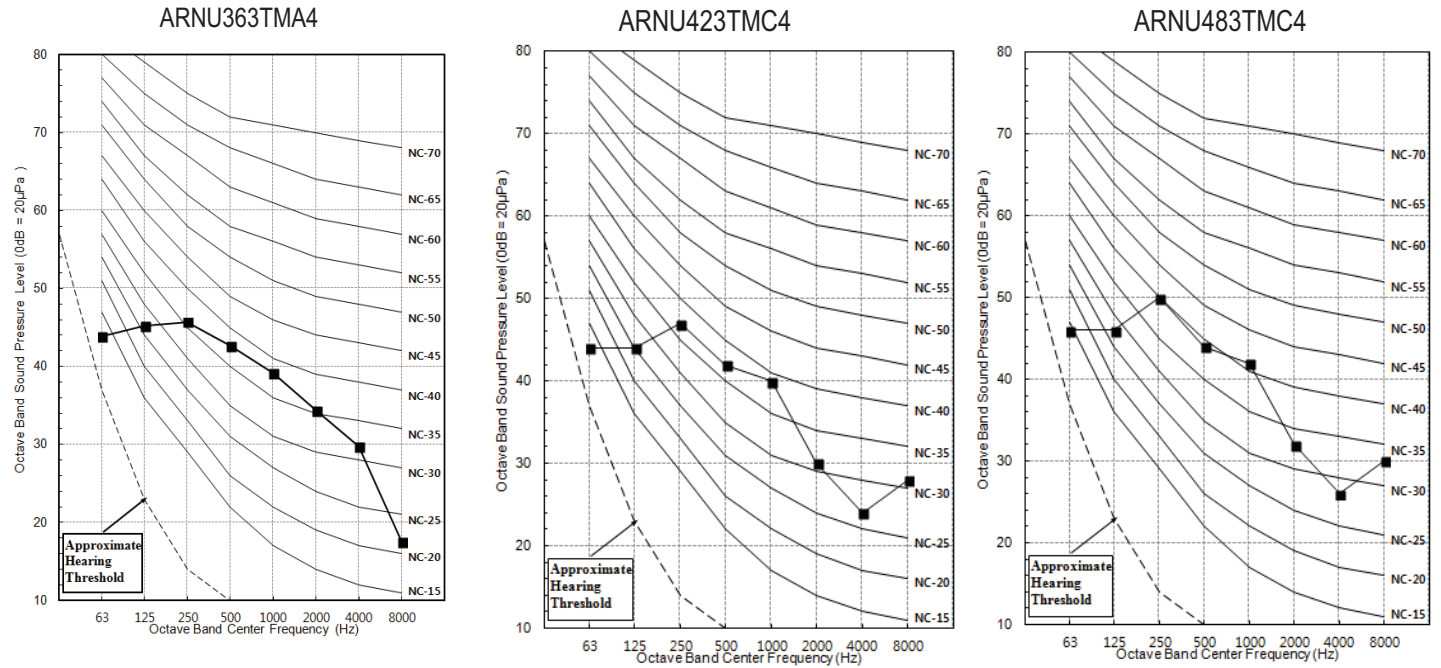
Figure 43: ARNU363TMA4, ARNU423TMCA, and ARNU483TMCA Sound Pressure Level Diagrams.
