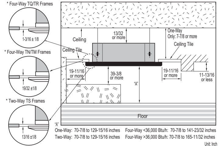
Figure 83: Selecting the Best Location / Minimum Clearance Requirements — One-, Two-, and Four-Way Ceiling-Cassette Indoor Units.
