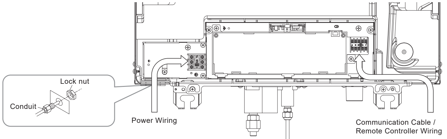
Figure 96: Typical TS Frame Wiring / Cable Routing.
