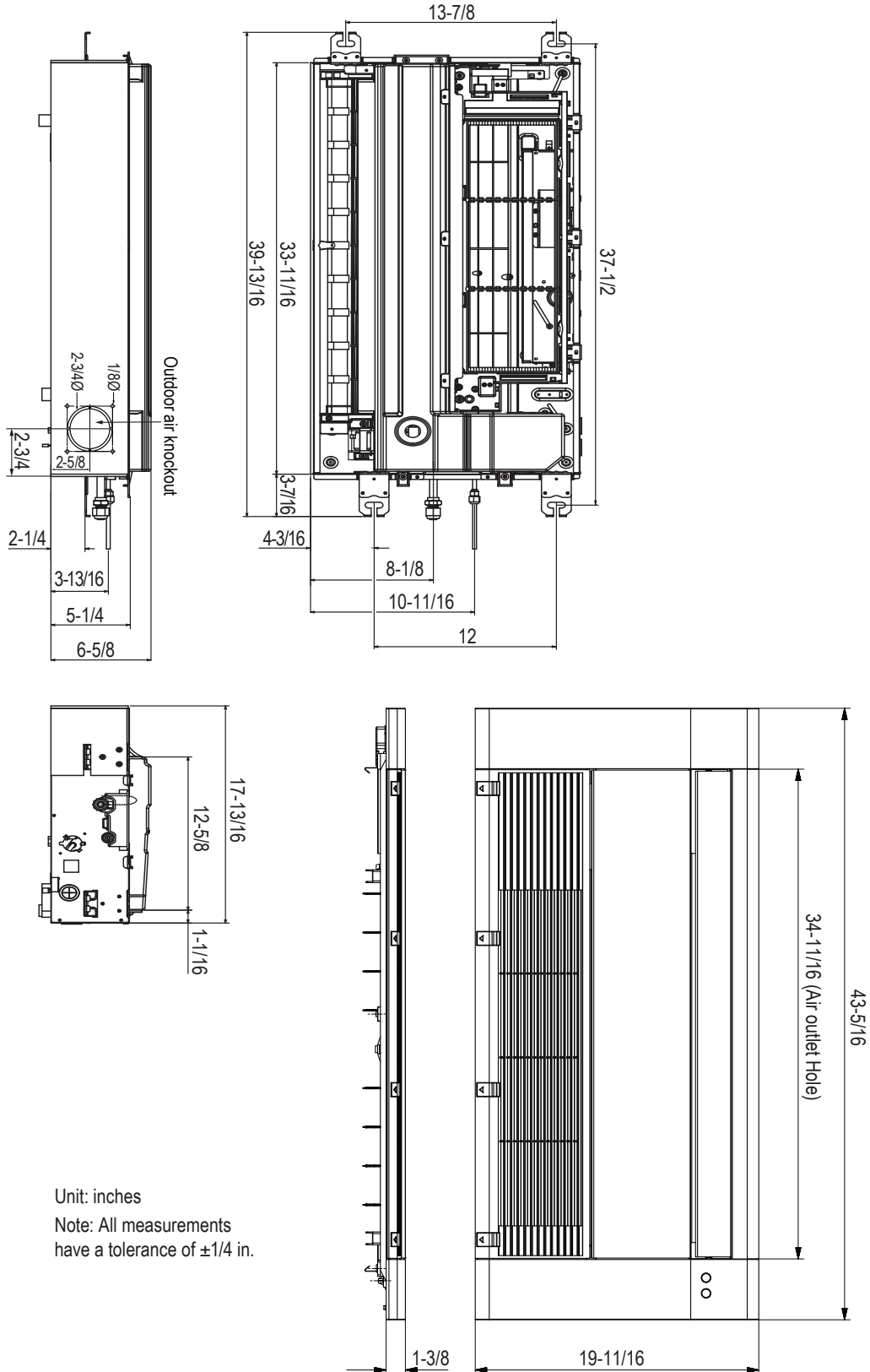
Figure 3: ARNU073TUD4, ARNU093TUD4, ARNU123TUD4 Dimensions (PT-UUC1 Grille).
