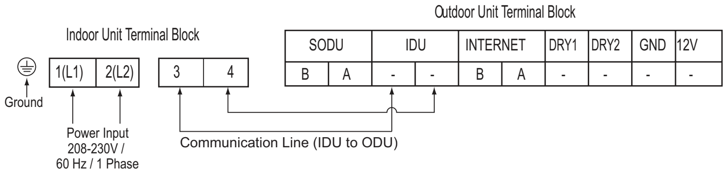
Figure 94: TT, TU Frame Wiring / Cable Connections.
