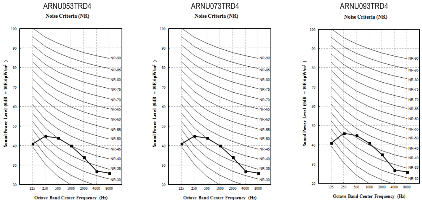
Figure 44: ARNU053TRD4, ARNU073TRD4, and ARNU093TRD4 Sound Power Level Diagrams.
