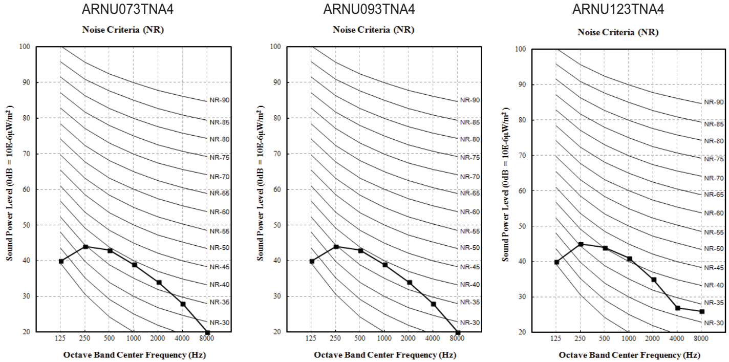
Figure 46: ARNU073TNA4, ARNU093TNA4, and ARNU123TNA4 Sound Power Level Diagrams.
