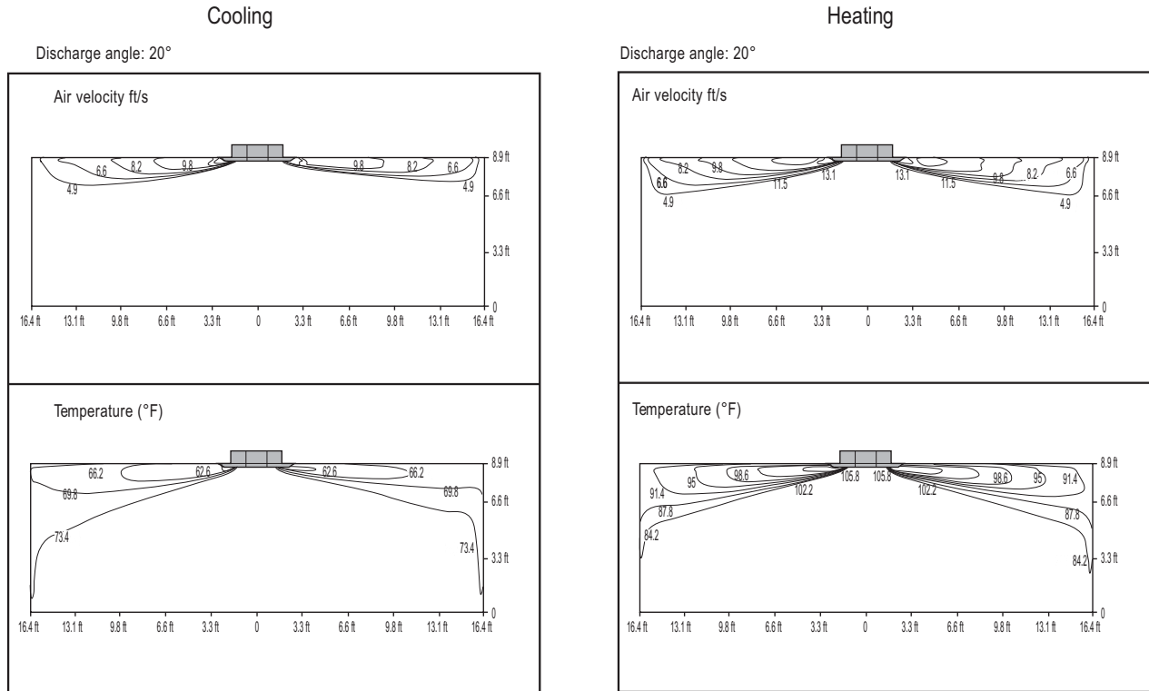
Figure 71: ARNU283TMA4.
