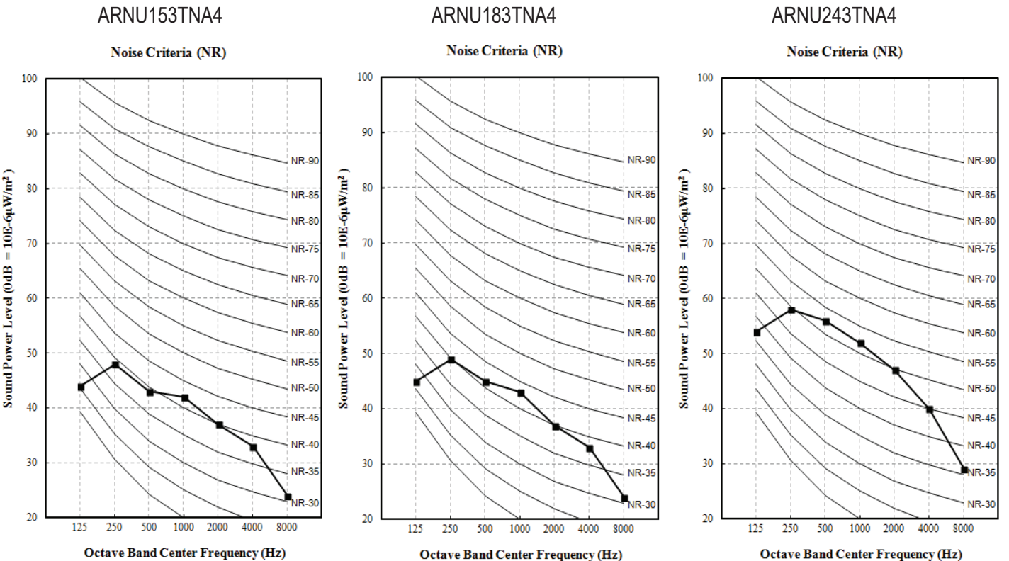
Figure 47: ARNU153TNA4, ARNU183TNA4, and ARNU243TNA4 Sound Power Level Diagrams.
