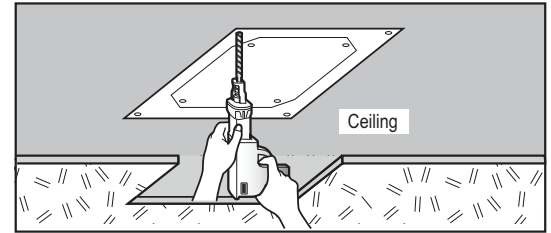
Figure 88: Using the Paper Pattern / Drilling Holes for the Bolts, Refrigerant and Condensate Piping.
