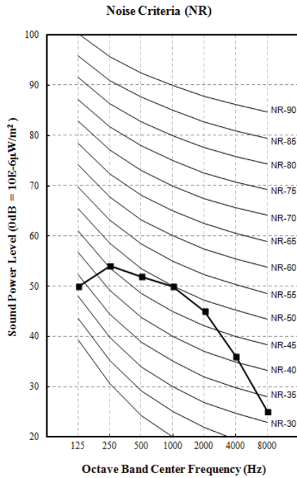
Figure 49: ARNU363TMA4 Sound Power Level Diagram.
