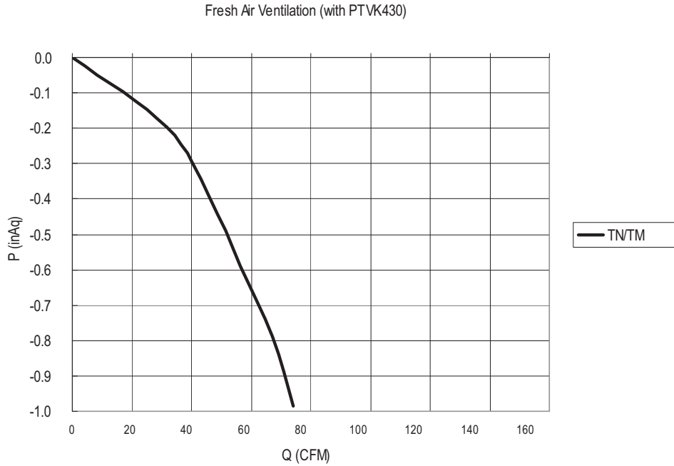
Figure 81: TN and TM Frame Fresh Air Ventilation with PTVK430 Accessory.
