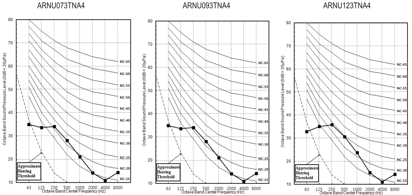
Figure 40: ARNU073TNA4, ARNU093TNA4, and ARNU123TNA4 Sound Pressure Level Diagrams.
