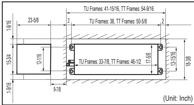
Figure 85: Ceiling Opening / Hanging Bolt Locations for One-Way Ceiling Cassette Indoor Units.
