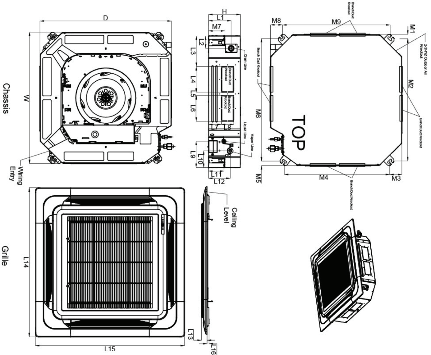
Figure 33: ARNU283TMA4, ARNU363TMA4, ARNU423TMC4, and ARNU483TMC4 Dimensions.
