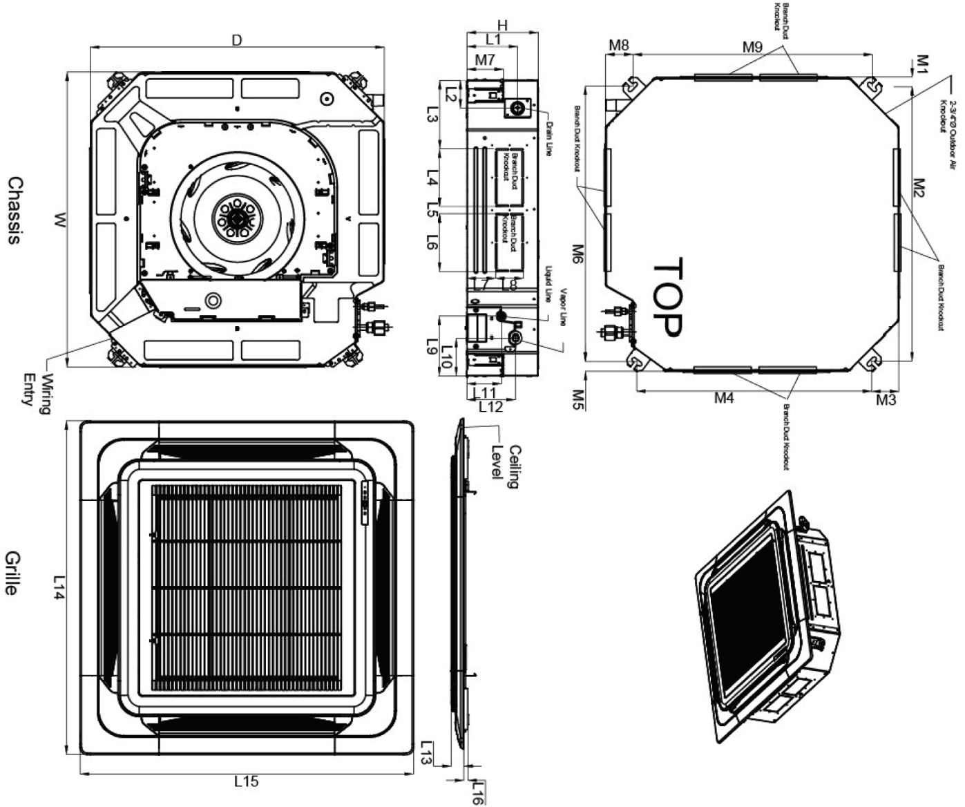
Figure 32: ARNU073TNA4, ARNU093TNA4, ARNU123TNA4, ARNU153TNA4, ARNU183TNA4, and ARNU243TNA4 Dimensions.
